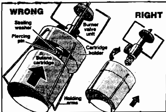
Wrong: The cartridge is fitted into the assembled appliance and pierced without being held securely in place. Right: The butane cartridge should be placed into its holder before it is attached to the valve unit and then pierced.
